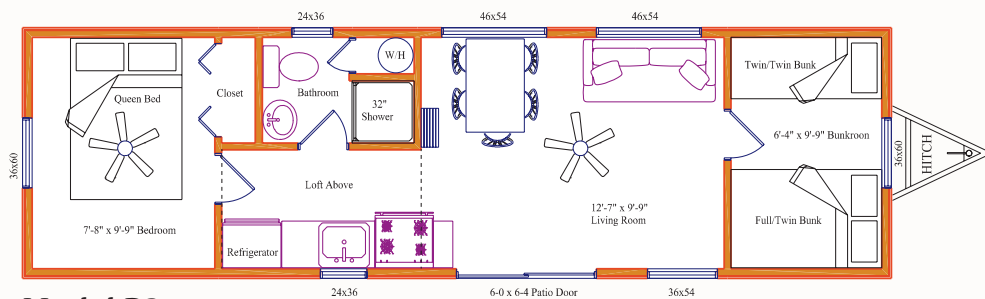
Model P37 - Size: 10'-6" x 37', 2 Bedroom, Loft
